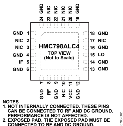
Figure 2. Pin Configuration
